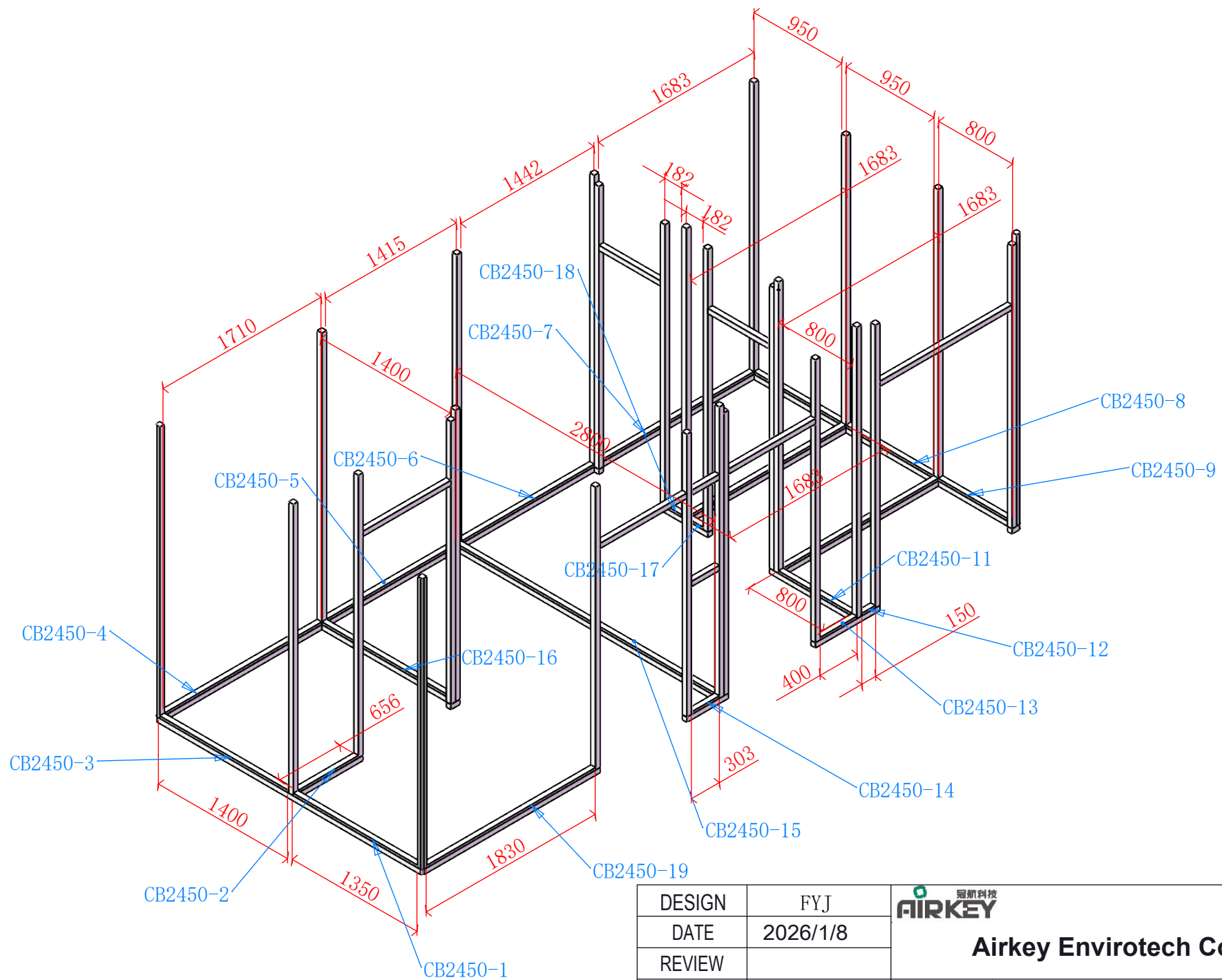
BRACING FRAME ASSEMBLY
